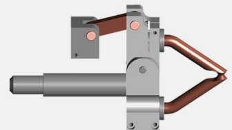
13.PS.11.55 G to C Adapter (G Clamp)
